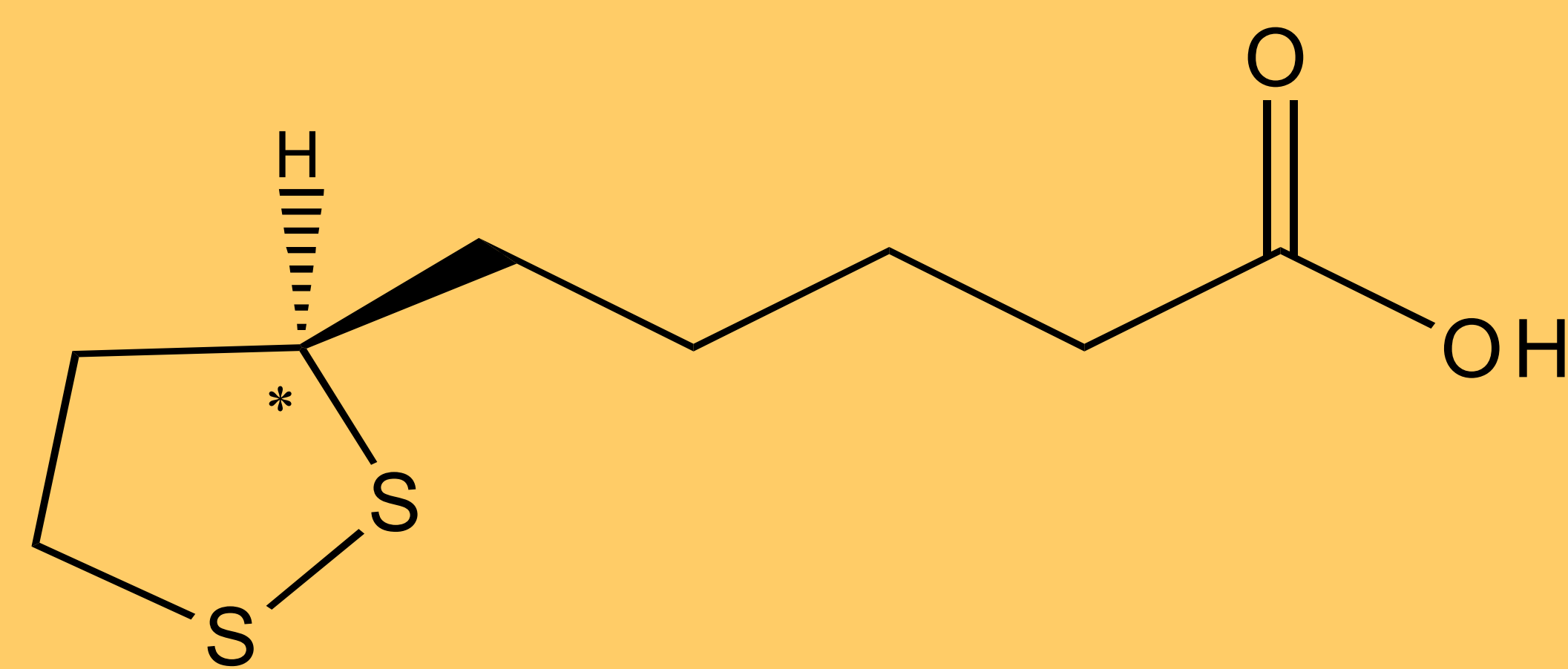
R-(+)-lipoic acid [1200-22-2]
